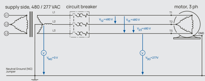
Figure 4: Simplified wye-configured, 480/277 V three-phase system
