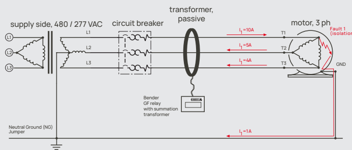
Figure 5: Faulted three-phase grounded system with zero-sequence relay
