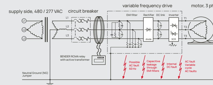
Figure 7: Grounded system with variable frequency drive
