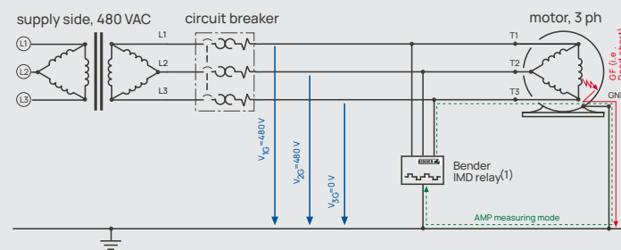
Figure 2: Ungrounded three-phase system with IMD
