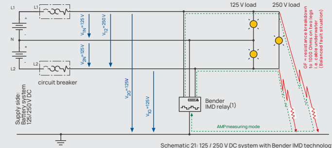
Figure 3: 125/250 VDC ungrounded system with IMD
