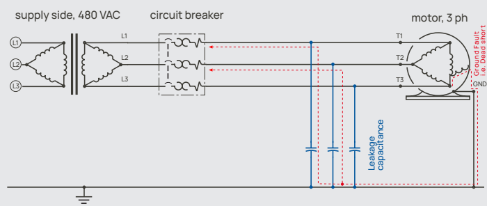
Figure 1: Ungrounded system in single-fault condition
