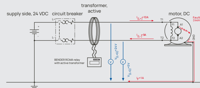
Figure 6: Grounded DC power system
